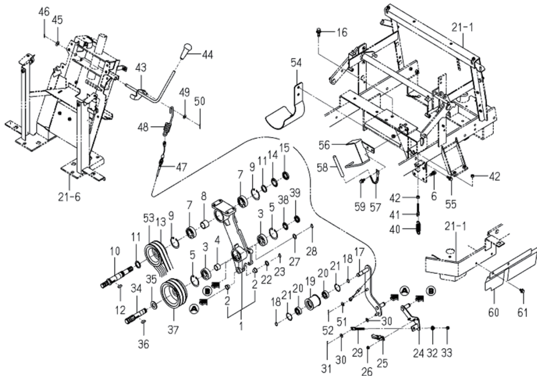
FIG.219 PTO(MOWER)SYSTEM
