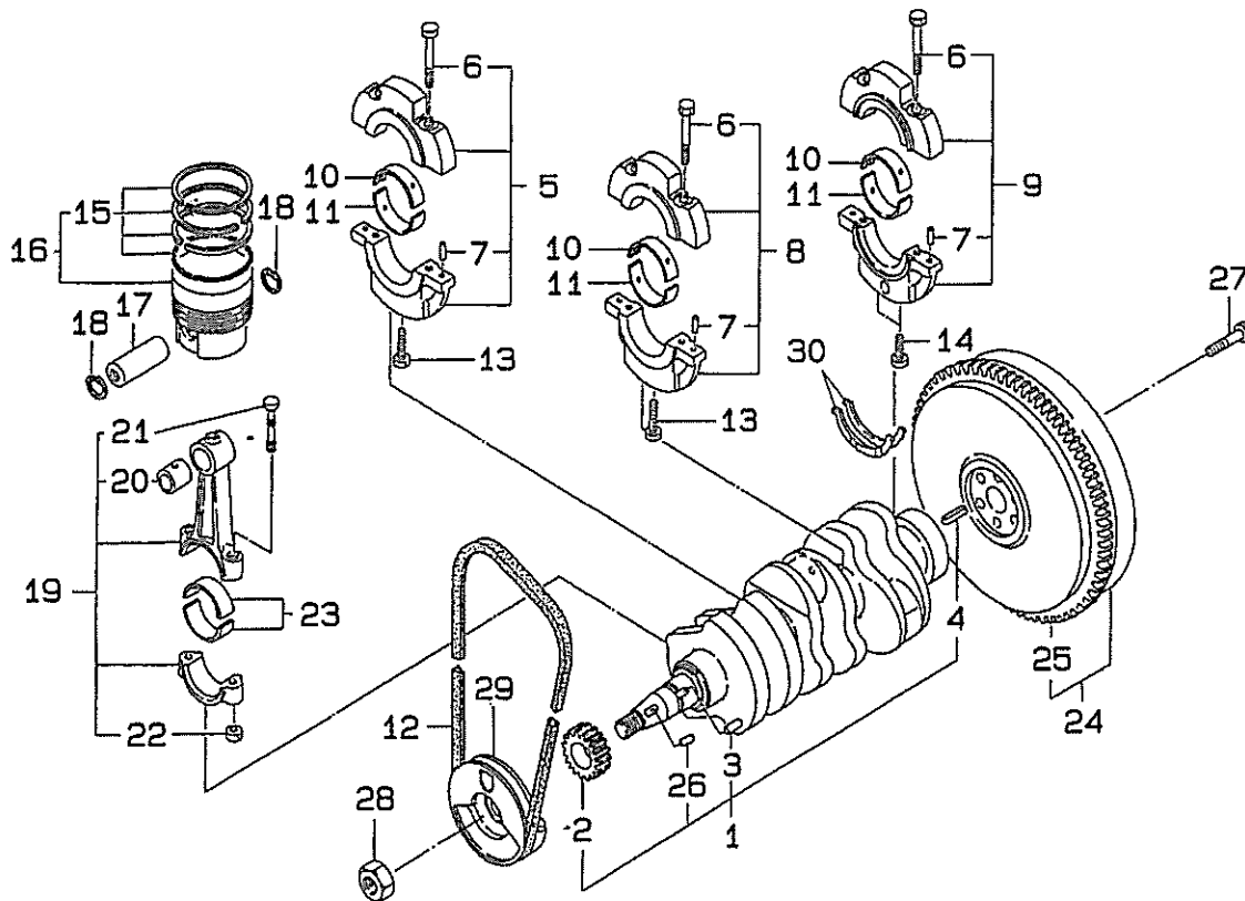
CRANK SHAFT
