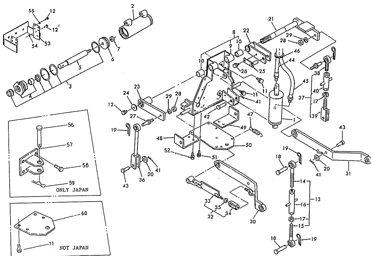
FIG.224 三点ヒッチ THREE-POINT LINKAGE
