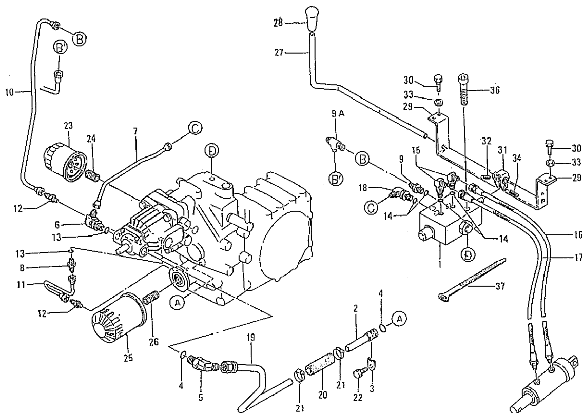
FIG.215 油圧配管 HYDRAULIC PIPING
