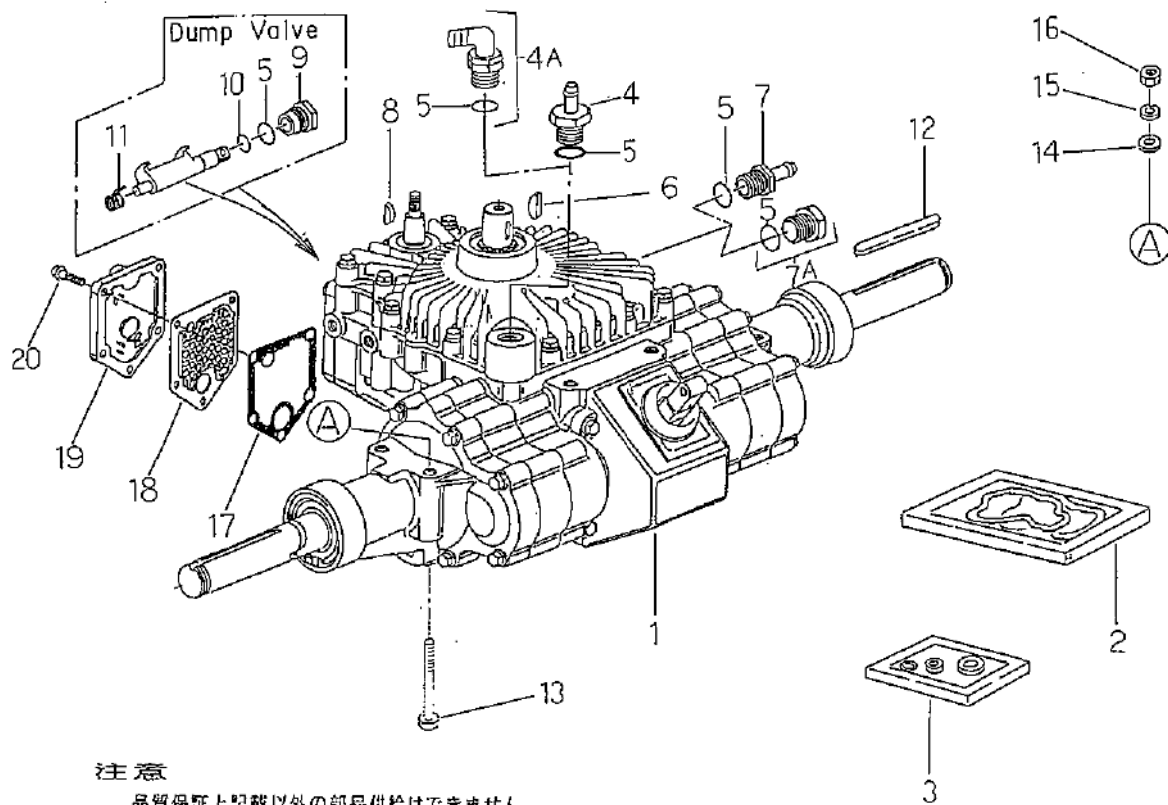
FIG.205 H.S.T HYDRAU STATIC TRANSMISSION
