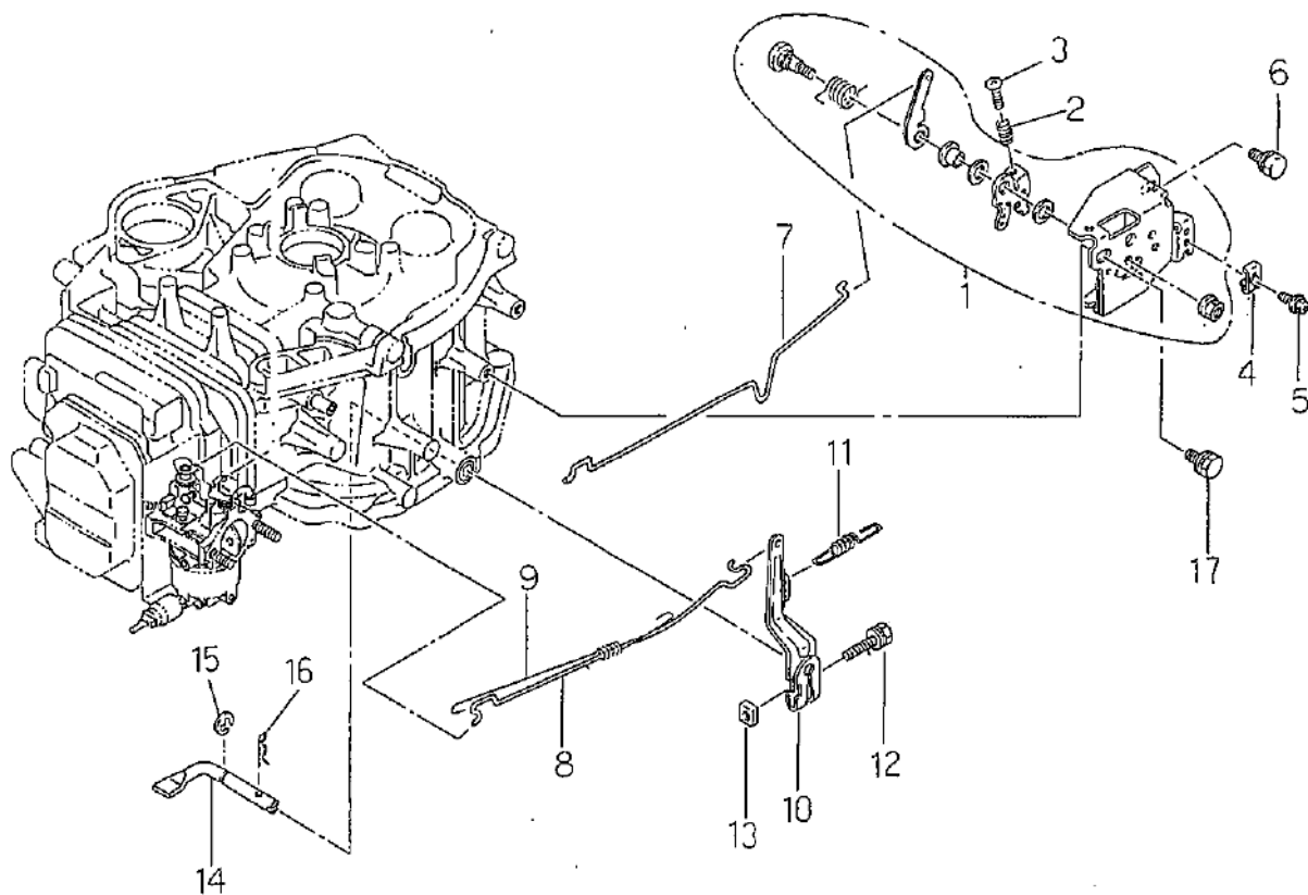
ガバナ GOVERNOR
